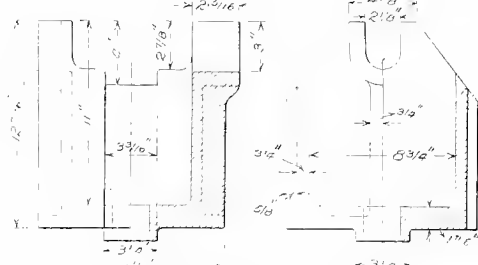
Figs. 4796-4797. Sectional End and Side Elevations.
